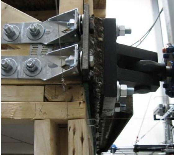
Example of Lateral Load Application Along Truss Bottom Chord [Note: Photo Taken During Testing]
