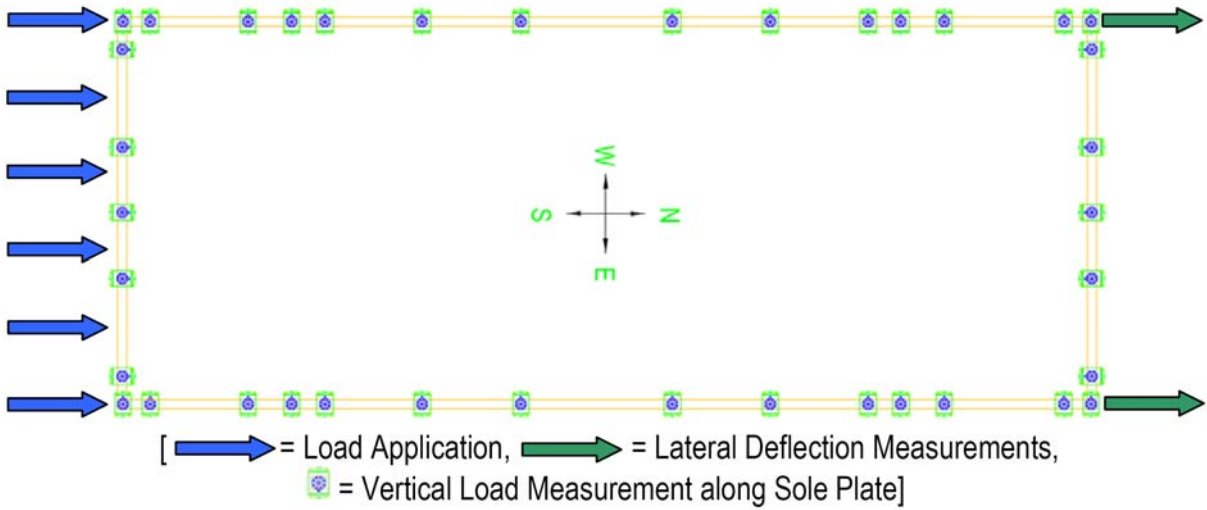
Plan View of Tests
